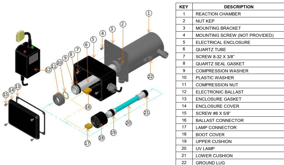
Figure 1: Exploded View
