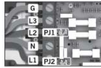
3 phase connection
