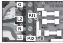
2 phase connection
